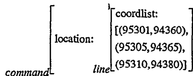
Figure 11: Line Interpretation of Gesture
