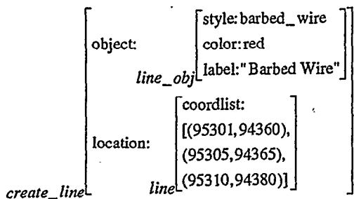
Figure 12: Feature Structure for Multimodal Line Creation
